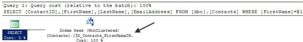
Figure 8-31. Execution plan for Included Column pattern
