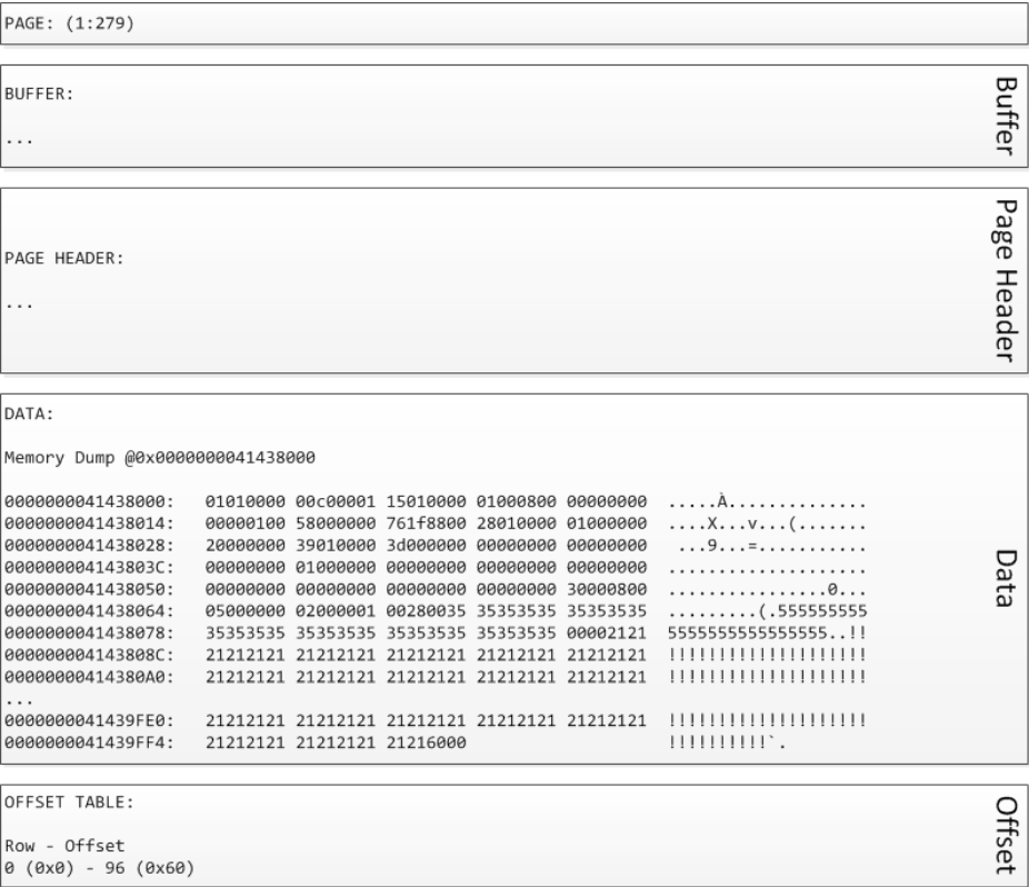
Figure 2-24. DBCC PAGE output for Hex Data Only print option
