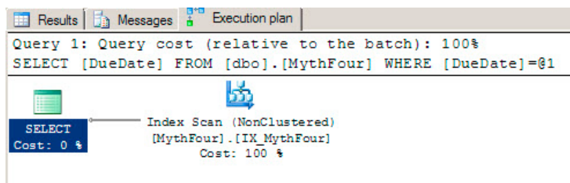
Figure 5-6. Execution plan for middle column in index
