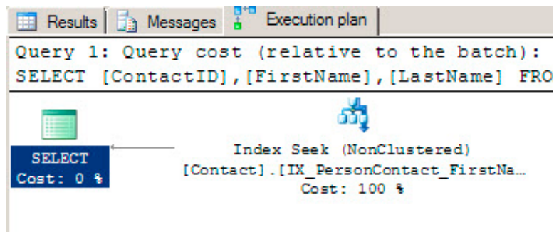
Figure 9-9. Execution plan with concatenation removed
