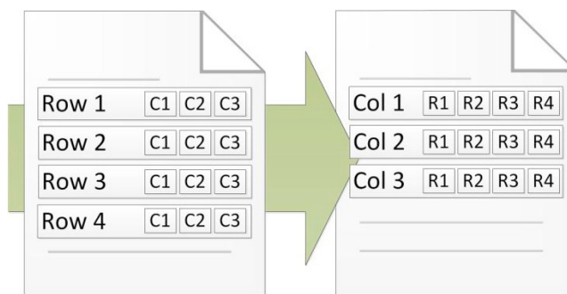
Figure 2-11. Row-wise vs. column-wise storage
