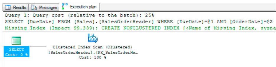
Figure 7-1. Execution plan for missing index SELECT query
