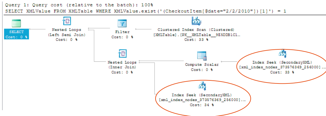
Figure 4-7. Execution plan results from the existence of a primary index and three secondary indexes
