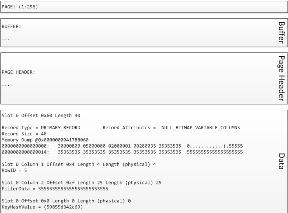
Figure 2-25. DBCC PAGE output for row data print option for data page
