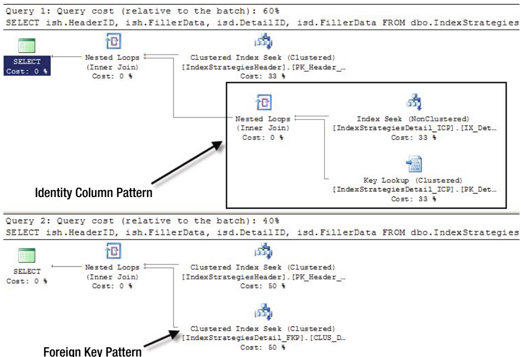
Figure 8-7. Execution plans for single header row on foreign key pattern
