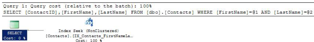
Figure 8-23. Execution plan for Multiple Columns pattern
