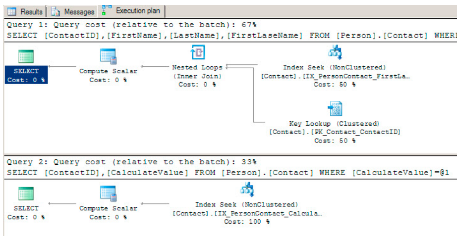
Figure 9-11. Indexed computed column execution plans
