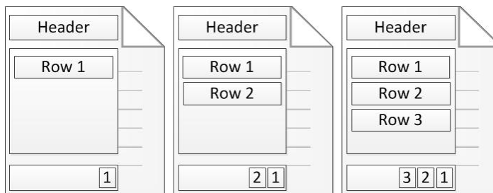
Figure 2-2. Row placement and offset array
